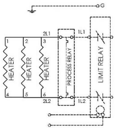
1-Phase Circuit
