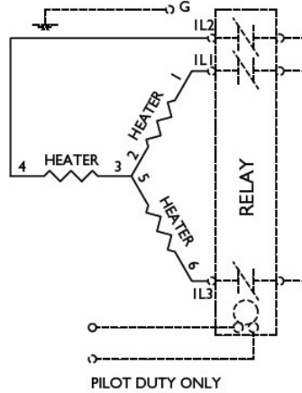
3-Phase Wye
