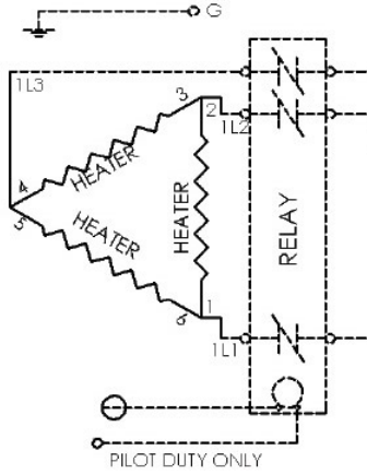
3-Phase Delta
