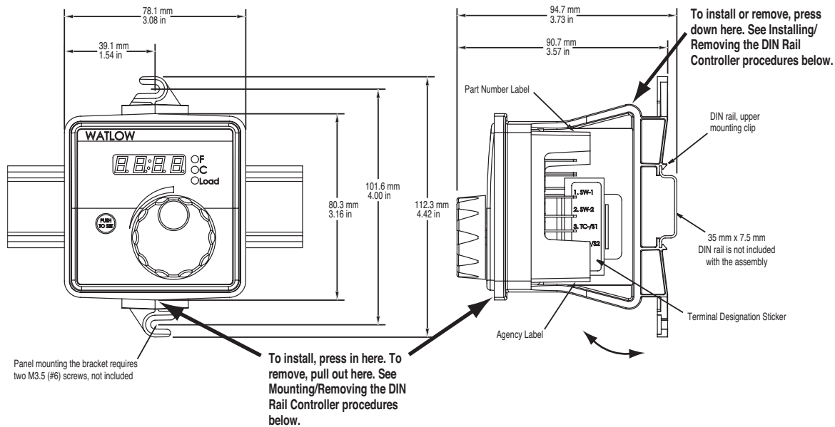
Figure 3a Sub-Panel Mounting
