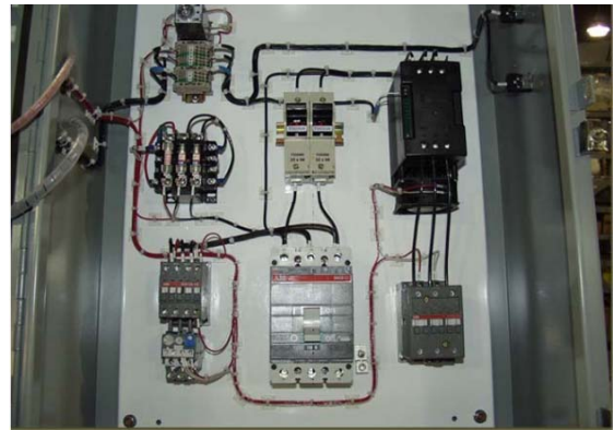
Internal View of a Control Panel
